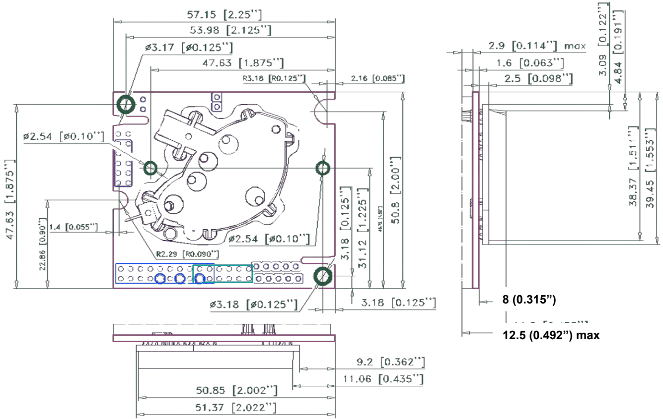
Figure 3. CO 2 Engine® K30 FR mechanical drawing.
