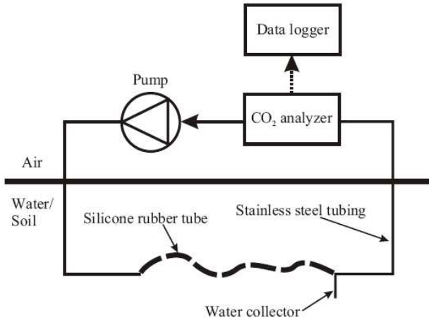
Figure 1. Schematic picture of the measurement setup.
